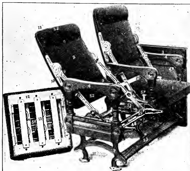
Fig. 3922. No. 61. RECLINING CAR-SEAT. High-back, Twin Tilting Seat, Without Leg-rest.
